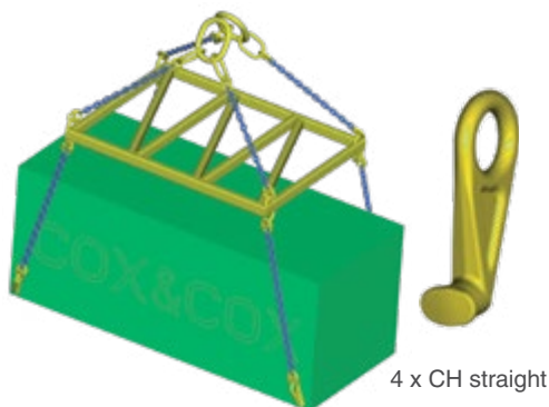
Alt. 1 - Straight lift
