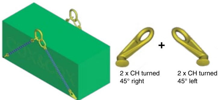
Alt. 2 - Angular lift
